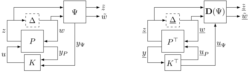
Fig. 2. Primal (left) and dual (right) controller interconnections.
